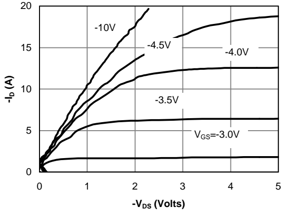
Fig 1: On-Region Characteristics
