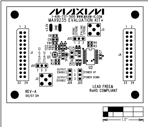
Figure 2. MAX9235 EV Kit Component Placement Guide—Component Side
