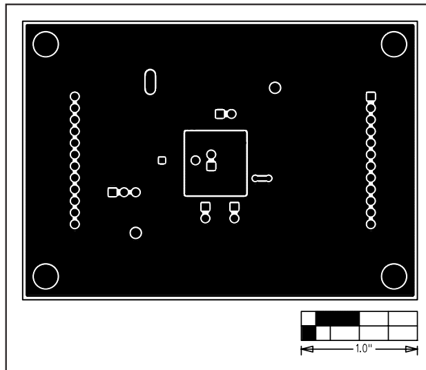
Figure 4. MAX9235 EV Kit PCB Layout—Solder Side
