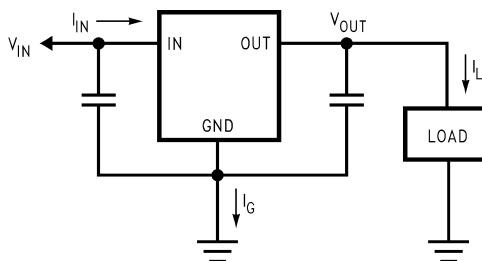
Figure 20. Power Dissipation Diagram
