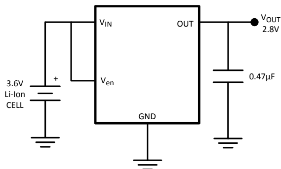
Figure 21. Single-Cell Regulator
