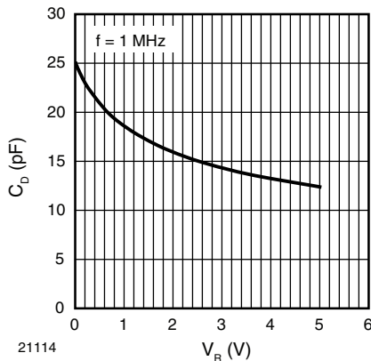
Fig. 3 - Typical Capacitance C_D vs. Reverse Voltage V_R
