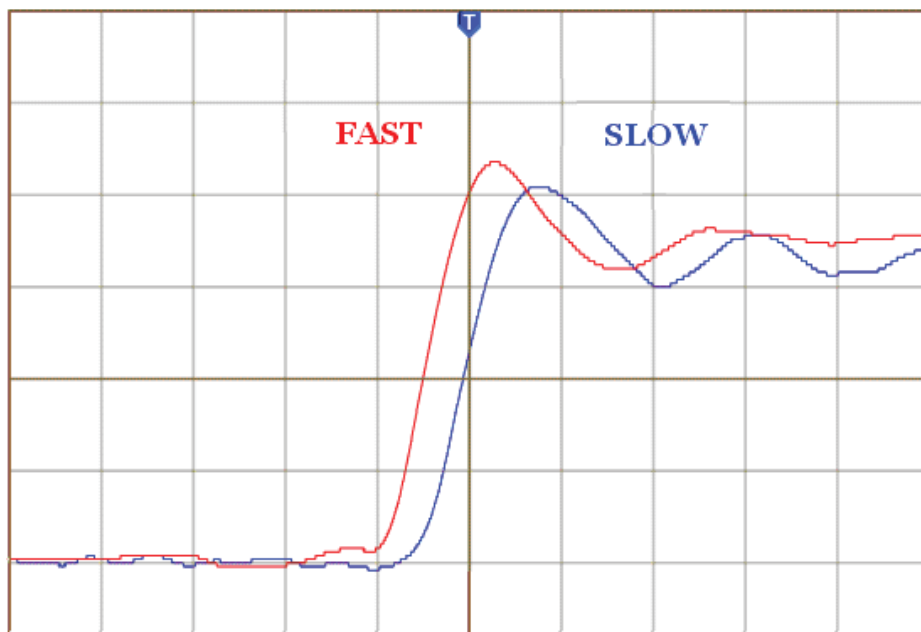
Figure 9: Slew Rate
