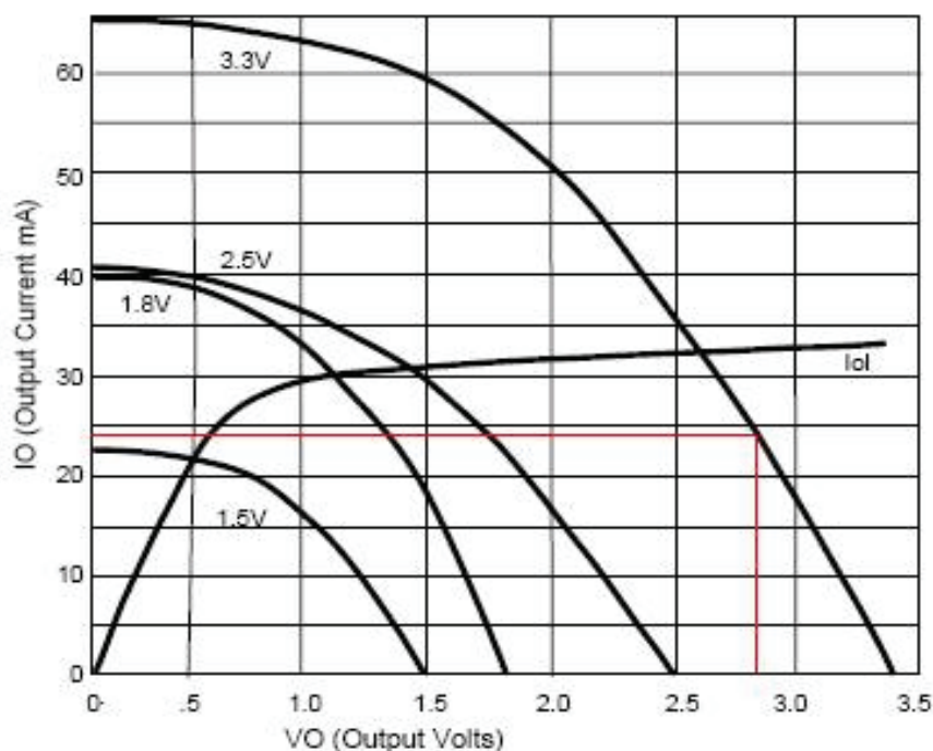
Typical I/V Curve for XC2C256
