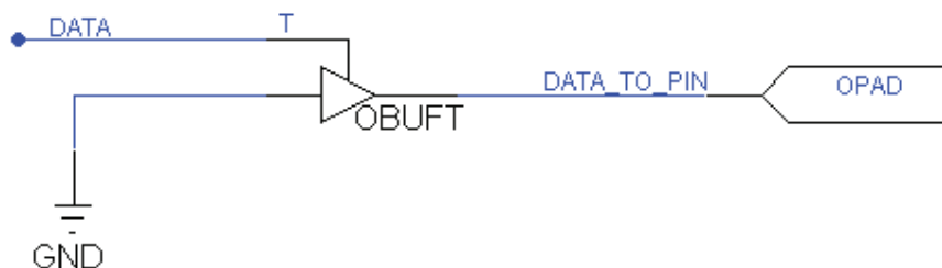
Figure 6: Simplified Method of Driving 5V
