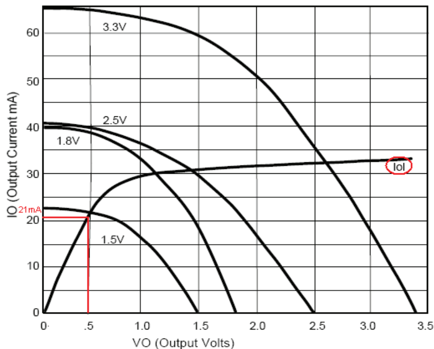
Typical I/V Curve for XC2C256
