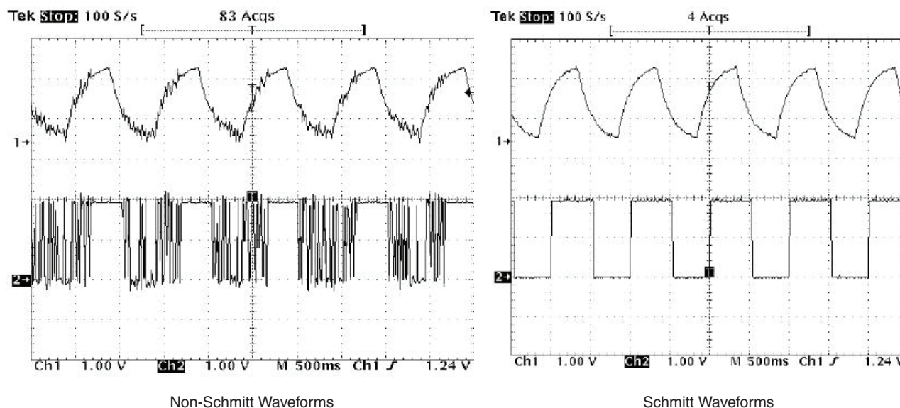
Figure 8: Before and After Schmitt Trigger Waveforms
