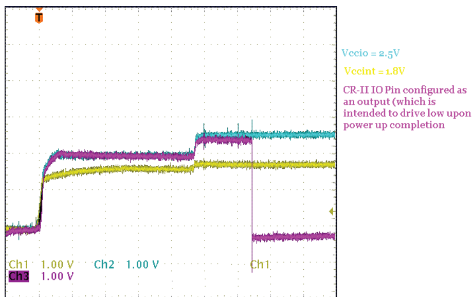
Figure 4: V_{CCINT} is powered after V_{CCIO}
