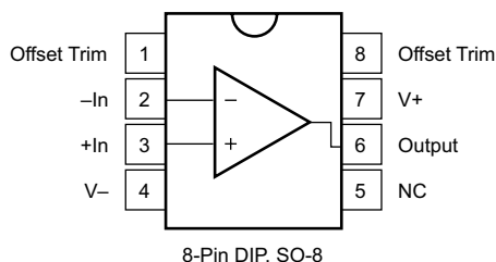
OPA132: P and D Packages 8-Pin PDIP and 8-Pin SOIC Top View
