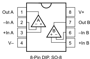
OPA2132: P and D Packages 8-Pin PDIP and 8-Pin SOIC Top View
