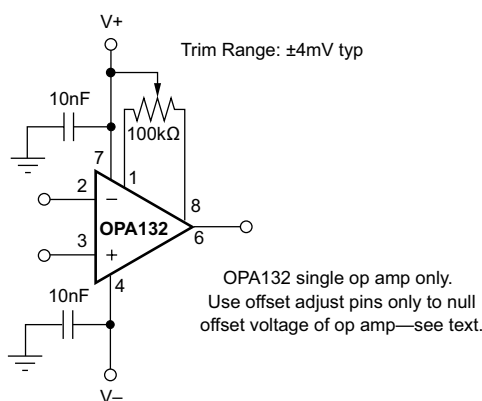
Figure 18. OPAx132 Offset Voltage Trim Circuit
