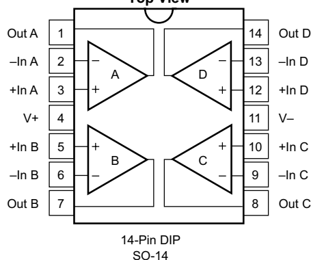
OPA4132: P and D Packages 14-Pin PDIP and 14-Pin SOIC Top View
