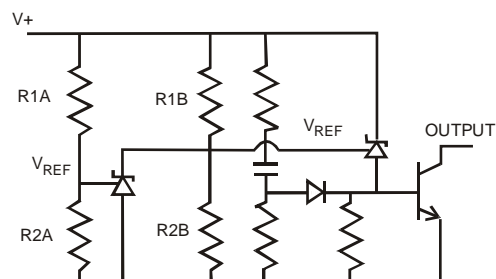
SERIES REGULATOR
