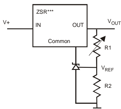
SHUNT REGULATOR
