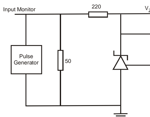
Test Circuit for Pulse Response
