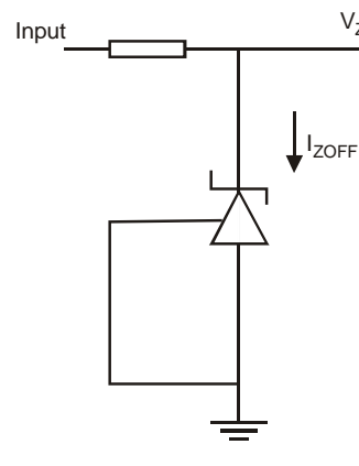
Fig.3 Test Circuit for Off State Current
