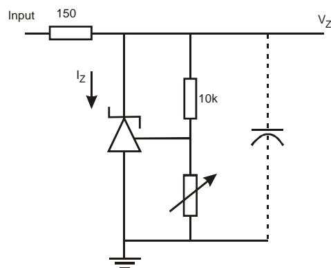
Test Circuit for Stability Boundary Conditions
