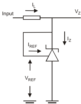
Fig. 1 Test Circuit for V_Z = V_{REF}
