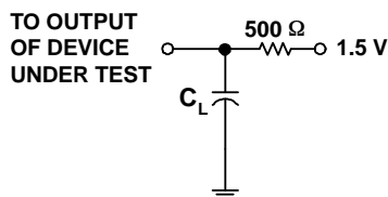
Figure 5. Receiver Disable Time ( t_{PHZ} , t_{PLZ} ) Test Circuit
