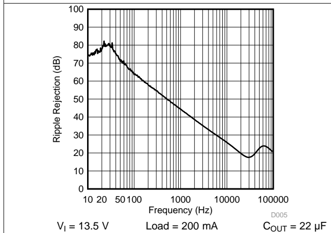
Figure 12. Power-Supply Ripple Rejection vs Frequency
