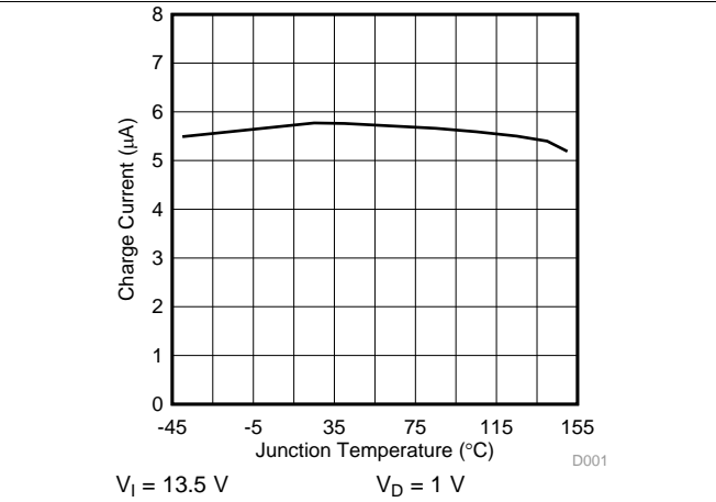
Figure 9. Charge Current ( I_{D,C} ) vs Junction Temperature
