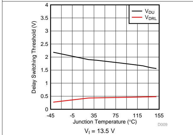
Figure 10. Delay Switching Threshold vs Junction Temperature
