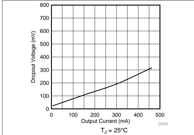
Figure 8. Dropout Voltage ( V_{do} ) vs Output Current
