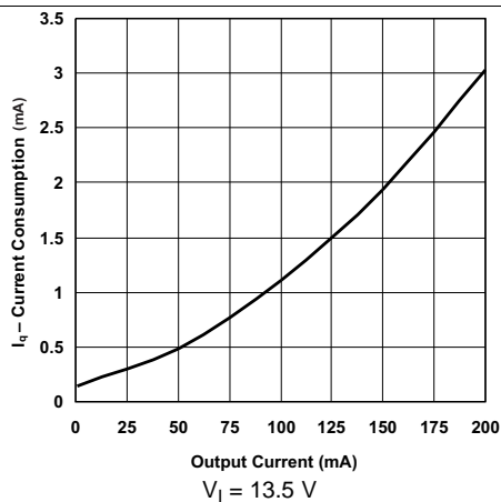
Figure 6. Current Consumption vs Output Current
