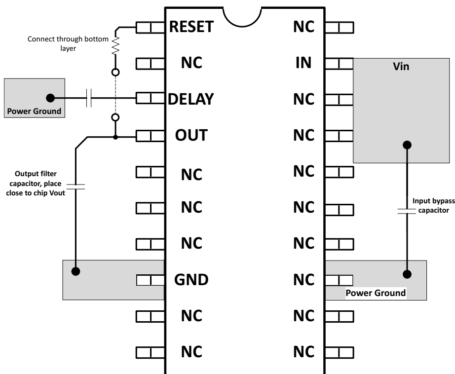
Figure 22. TLE4275-Q1 HTSSOP Layout Design Example
