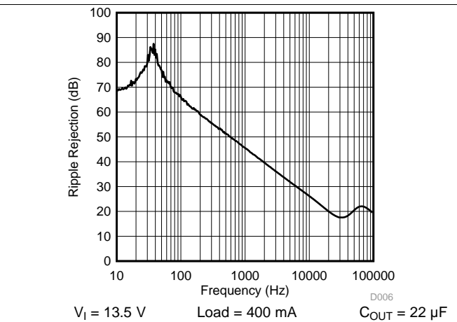
Figure 13. Power-Supply Ripple Rejection vs Frequency
