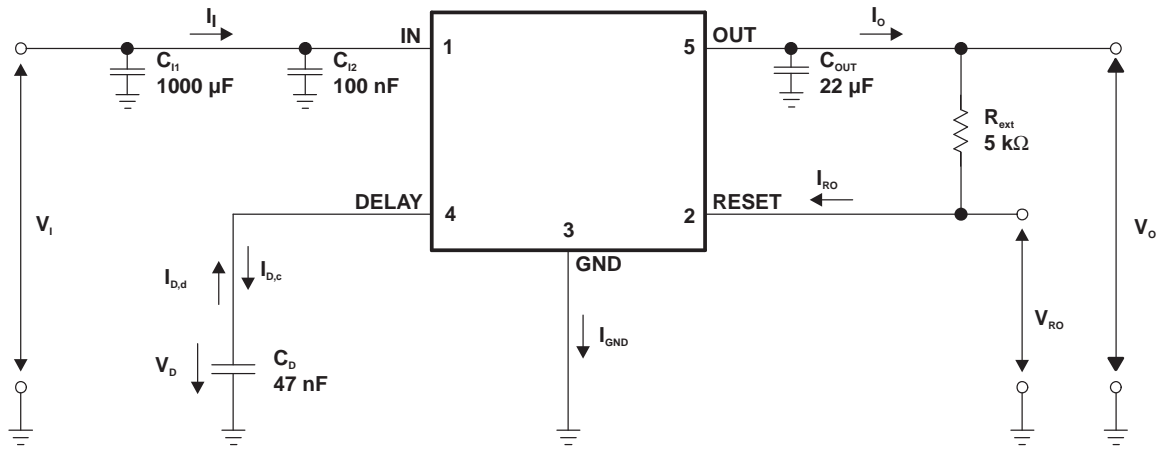
Figure 18. Test Circuit
