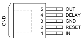
KTU Package 5-Pin DDPAK/TO-263 Top View
