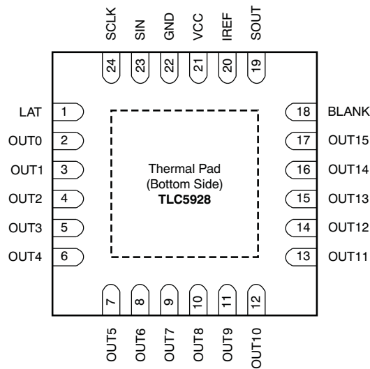
QFN-24 RGE PACKAGE (TOP VIEW)
