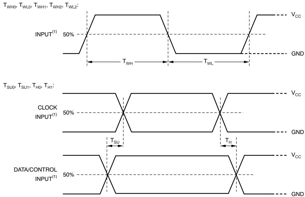
Figure 7. Input Timing
