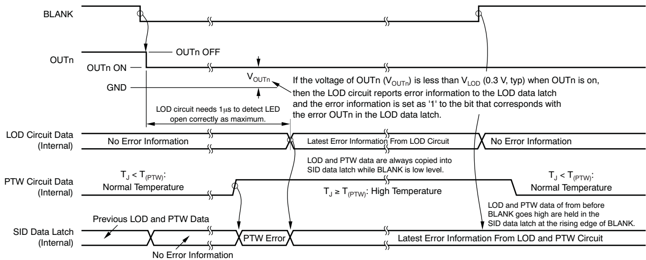
Figure 19. LOD/PTW/SID timing
