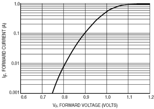
Figure 5. Forward Voltage
