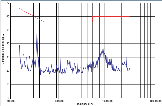
NPH25S4812
