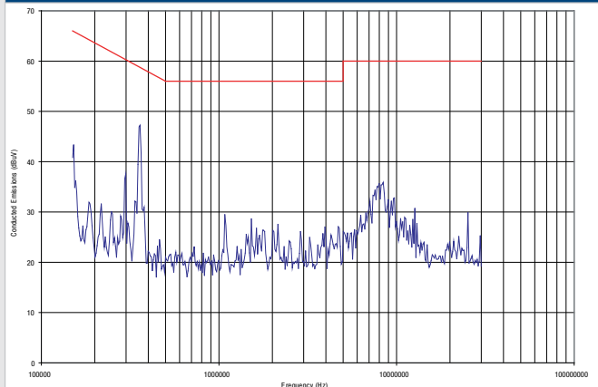
NPH25S4815
