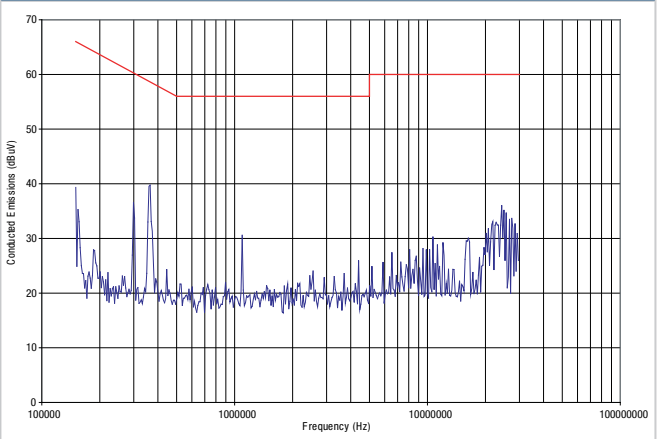
NPH25S2412
