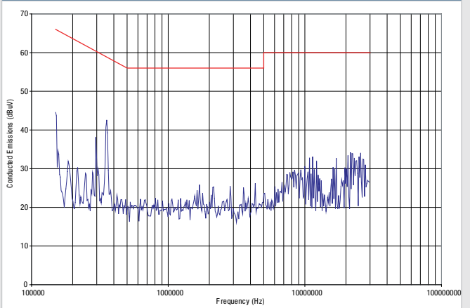
NPH25S2415
