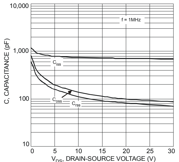
Fig. 6 Typical Capacitance
