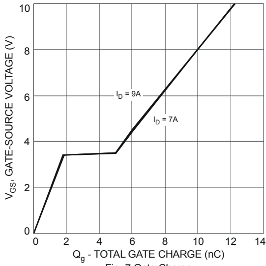
Fig. 7 Gate Charge
