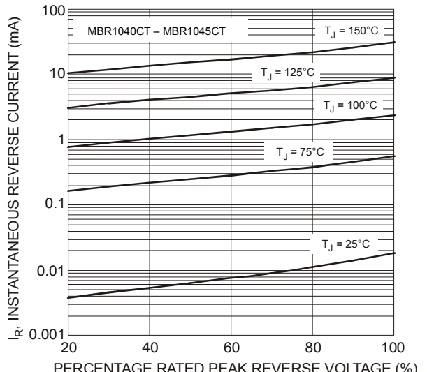
Figure 4 Typical Reverse Characteristics, per Element
