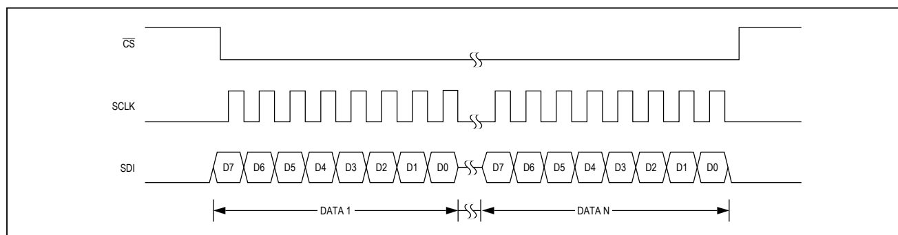
Figure 2. SPI Format
