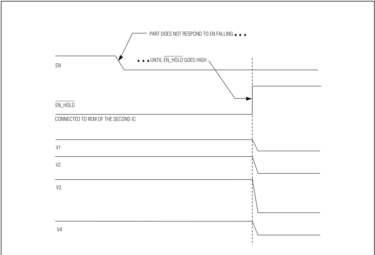
Figure 4. Power-Down Characteristics when REM of the Second IC is Connected to \overline{\text{EN\_HOLD}} of the First IC
