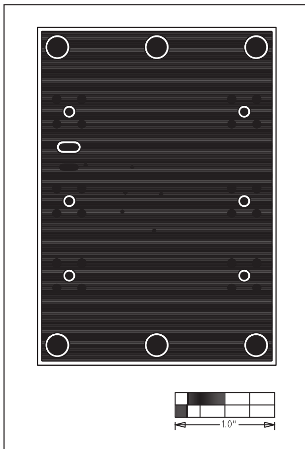
Figure 4. MAX9652 EV Kit PCB Layout—Solder Side
