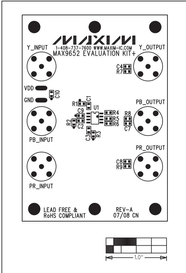
Figure 2. MAX9652 EV Kit Component Placement Guide—Component Side
