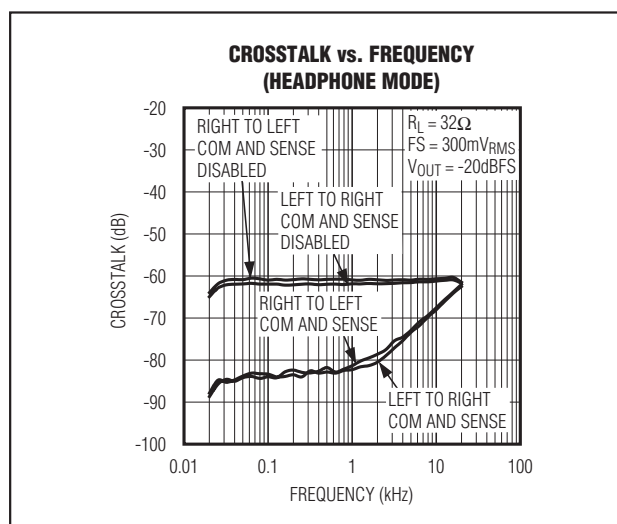
Figure 6. MAX9791/MAX9792 COM and SENSE Inputs Reduce Crosstalk
