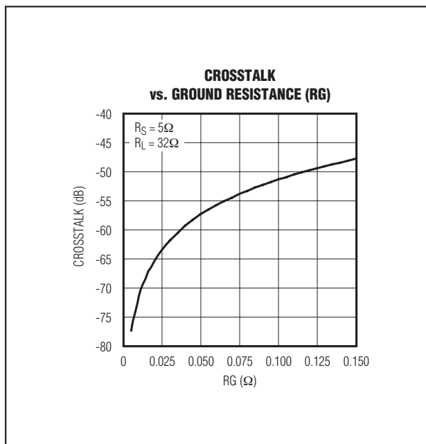
Figure 5. Crosstalk vs. Ground Resistance
