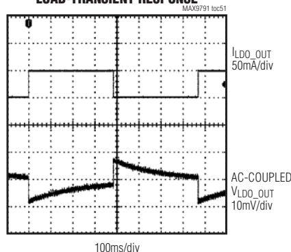
LOAD-TRANSIENT RESPONSE
