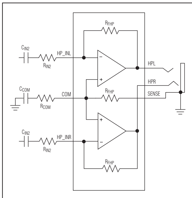
Figure 4. Connecting COM for Ground Sense
