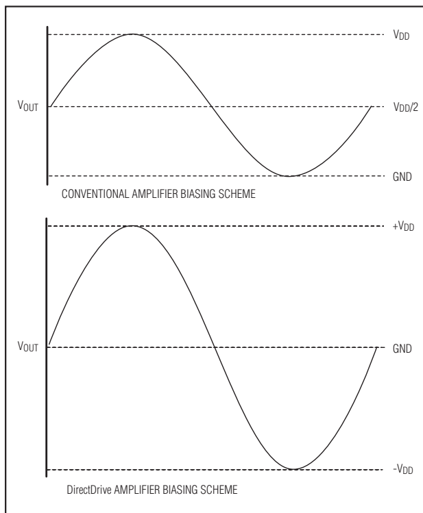
Figure 3. Traditional Amplifier Output vs. MAX9791/MAX9792 DirectDrive Output
