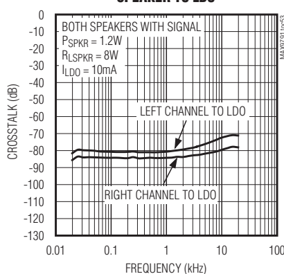
CROSSTALK vs. FREQUENCY SPEAKER TO LDO
