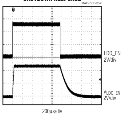
SHUTDOWN RESPONSE
