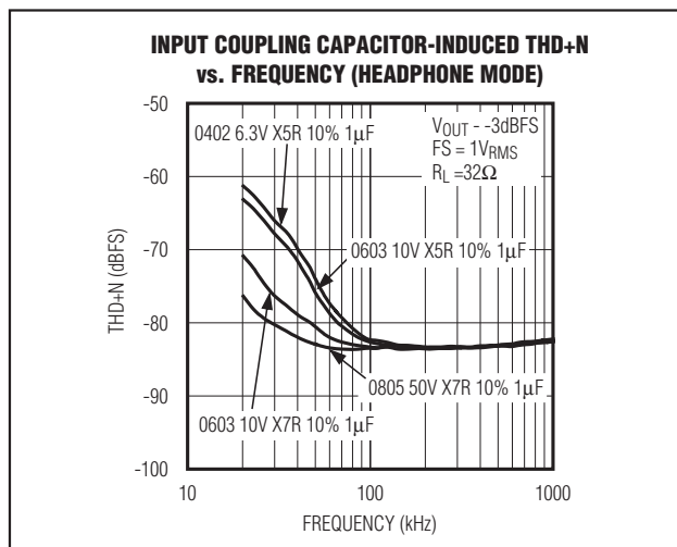
Figure 12. Input Coupling Capacitor-Induced THD+N vs. Frequency
