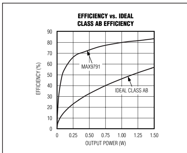
Figure 1. MAX9791 Efficiency vs. Class AB Efficiency
