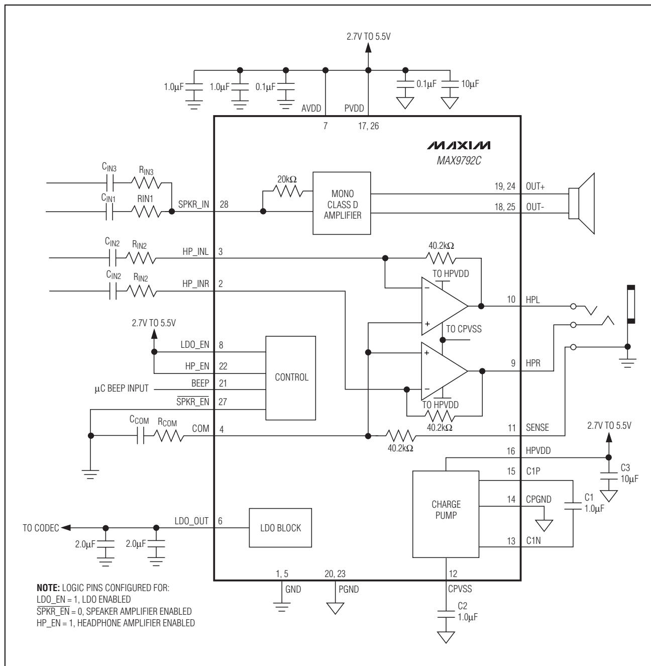
MAX9792C Block Diagram
