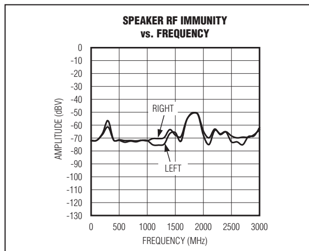
Figure 13. Speaker RF Immunity
