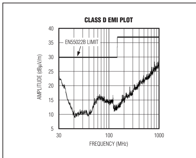
Figure 2. EMI with 30cm of Speaker Cable
