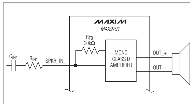
Figure 9. Setting Speaker Amplifier Gain
