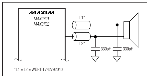
Figure 10. Optional Ferrite Bead Filter
