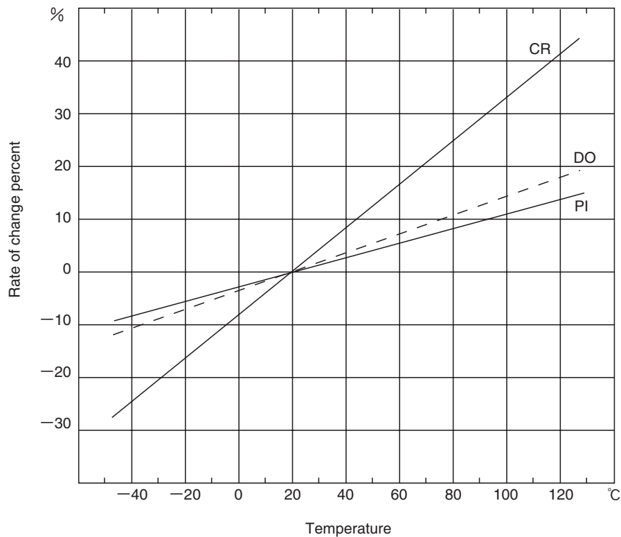
(1) Temperature characteristics
