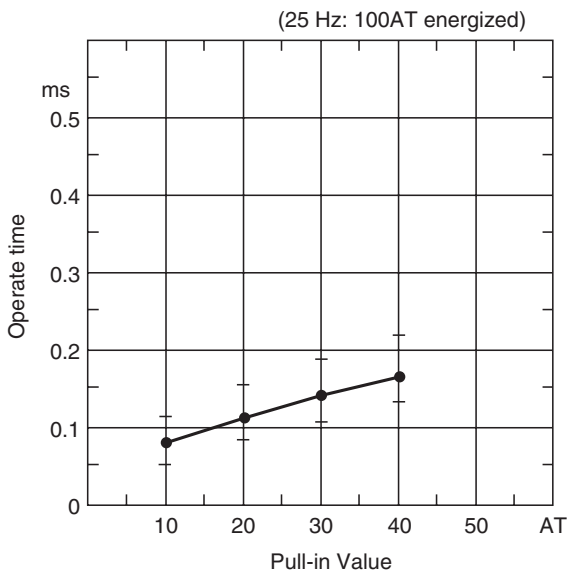
(1) Operate time
