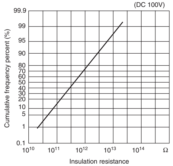
(4) Insulation resistance
