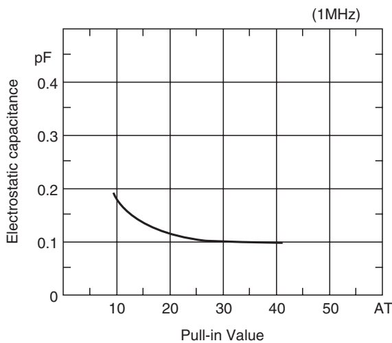
(5) Electrostatic capacitance
