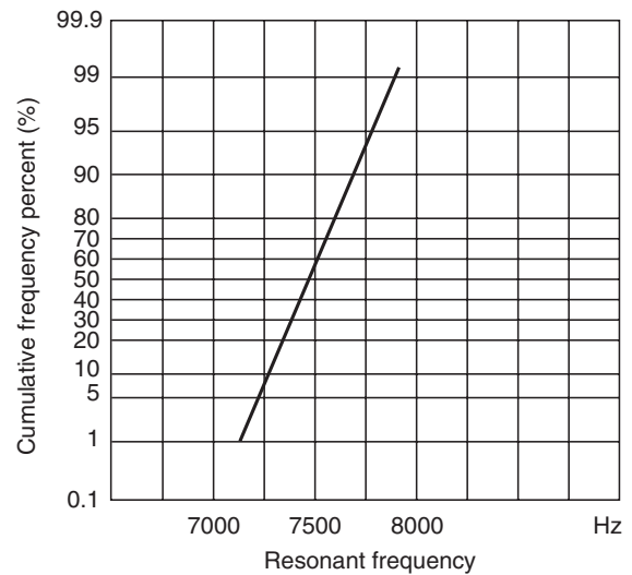
(4) Resonant frequency
