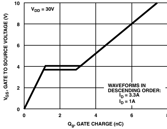
Figure 17. Gate Charge Waveforms for Constant Gate Currents
