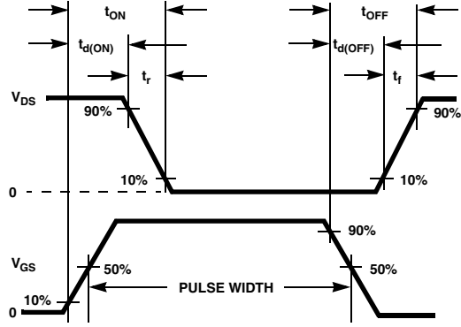
Figure 23. Switching Time Waveforms
