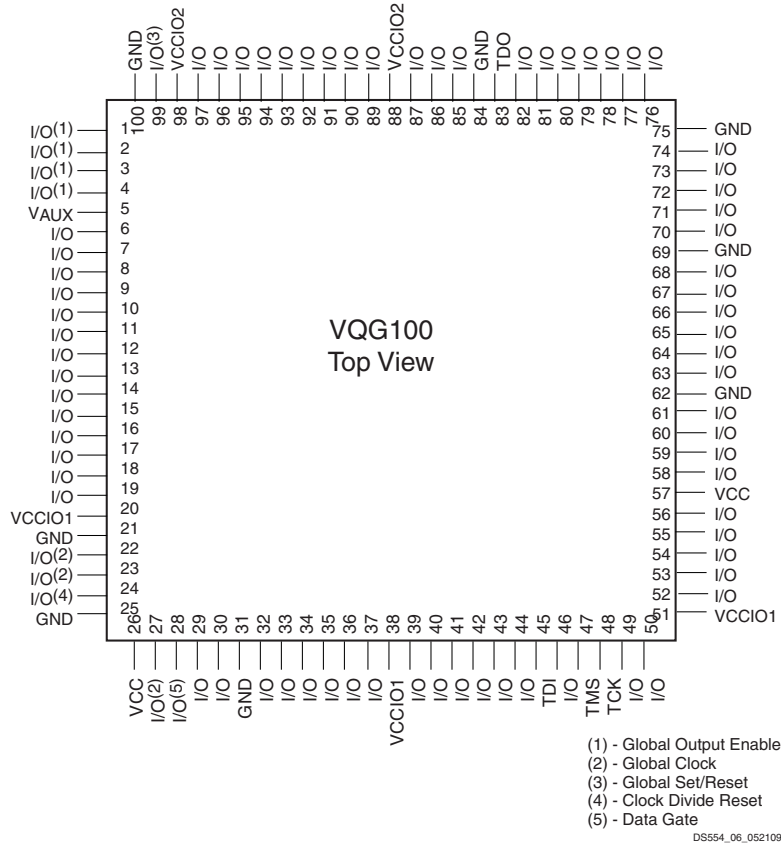
Figure 6: VQG100 Very Thin Quad Flat Pack
