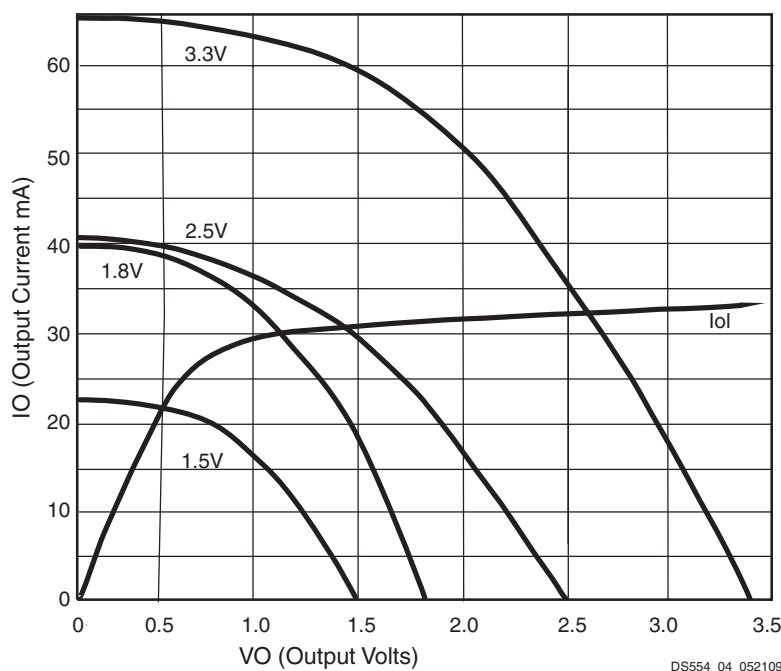
Figure 4: Typical I/V Curves for XA2C128
