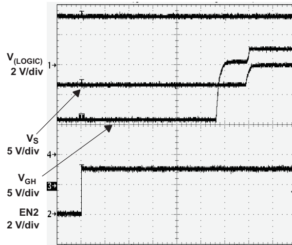
1 ms/div Figure 15.
