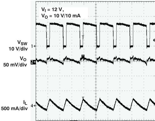
1 µs/div Figure 5.
