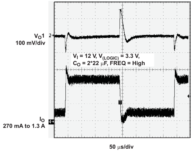
LOAD TRANSIENT RESPONSE STEP-DOWN CONVERTER
