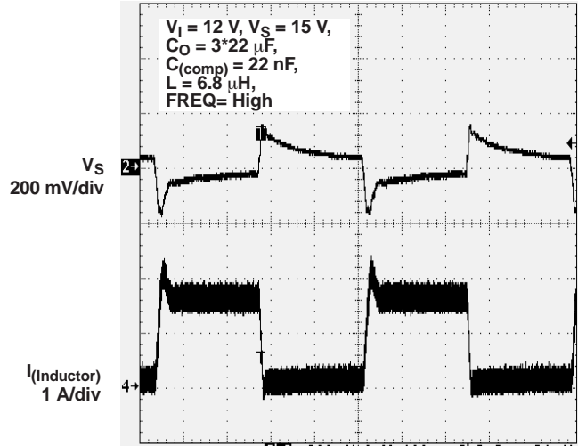
100 µs/div Figure 6.
