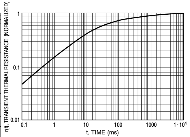
Figure 4. Thermal Response
