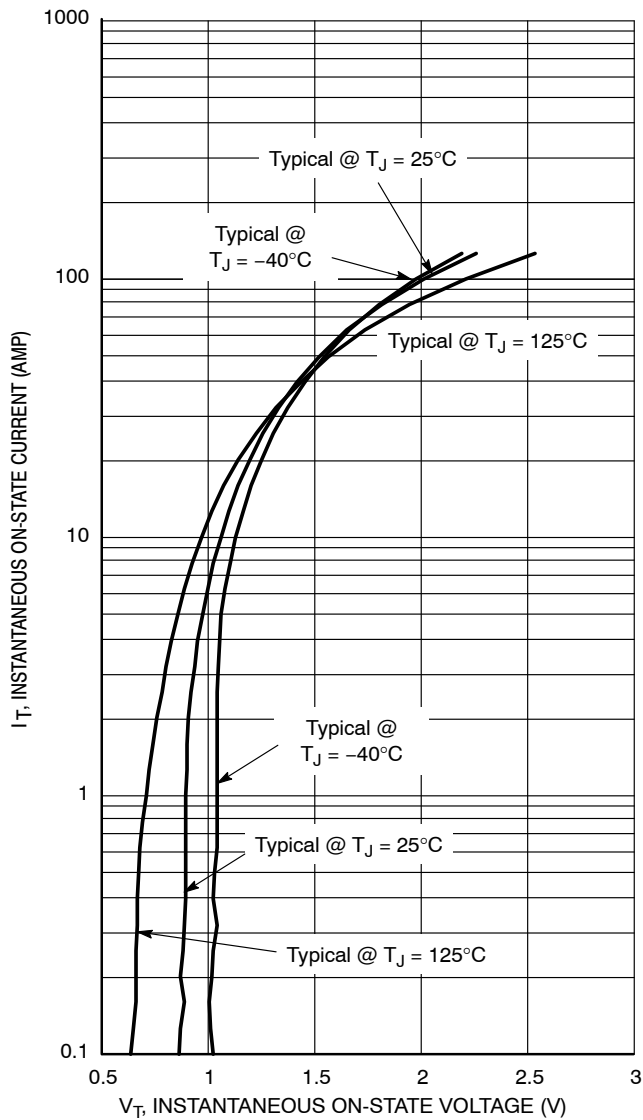
Figure 3. On-State Characteristics
