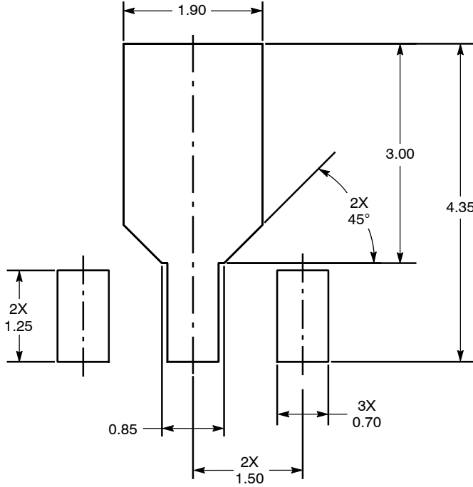
Figure 20. PCB Pad Layout for SOT-89A
