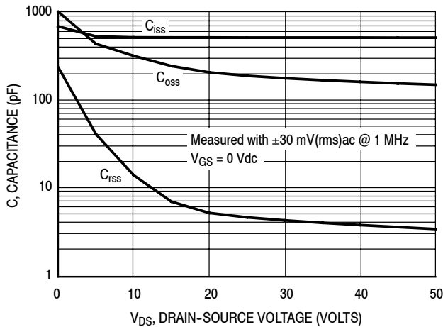
Figure 4. Capacitance versus Drain-Source Voltage
