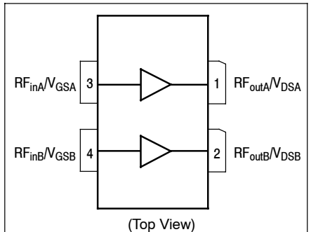
Figure 1. Pin Connections
