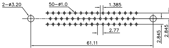
RECOMMENDED P.C.B LAYOUT (TOLERANCE +/-0.03)
