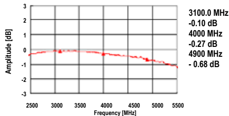
Amplitude Balance
