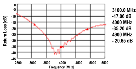
Return Loss
