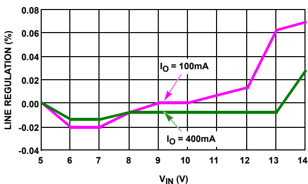
FIGURE 3. BOOST LINE REGULATION
