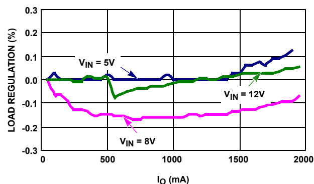
FIGURE 5. BUCK LOAD REGULATION
