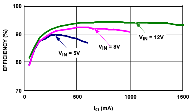
FIGURE 1. BOOST EFFICIENCY
