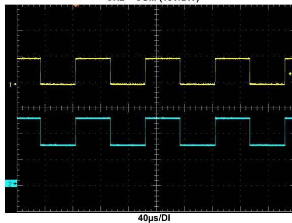
FIGURE 12. V_{ON} SLICE OPERATION
