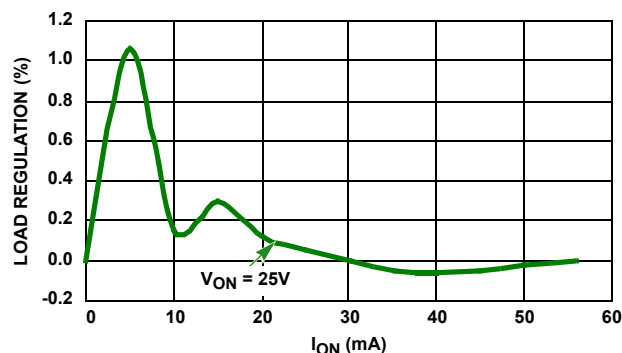
FIGURE 8. V_{OFF} LOAD REGULATION
