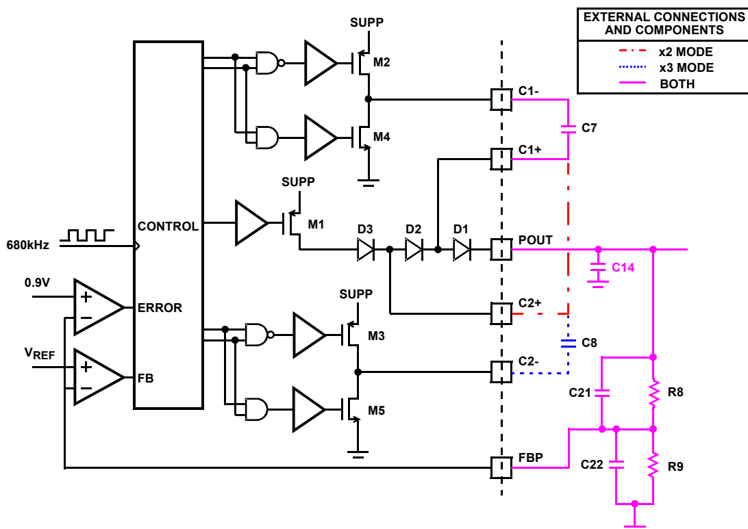
FIGURE 16. V_{ON} FUNCTION DIAGRAM
