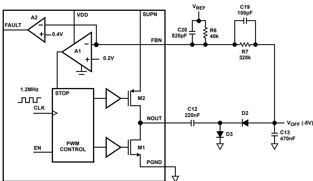
FIGURE 17. NEGATIVE CHARGE PUMP BLOCK DIAGRAM
