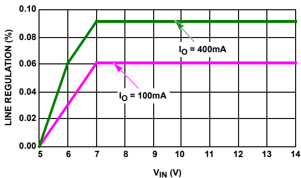
FIGURE 6. BUCK LINE REGULATION
