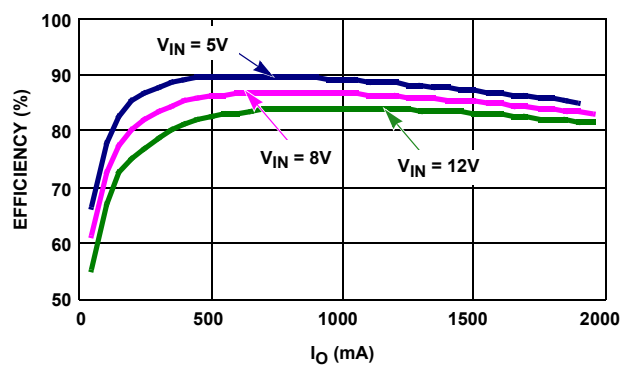
FIGURE 4. BUCK EFFICIENCY
