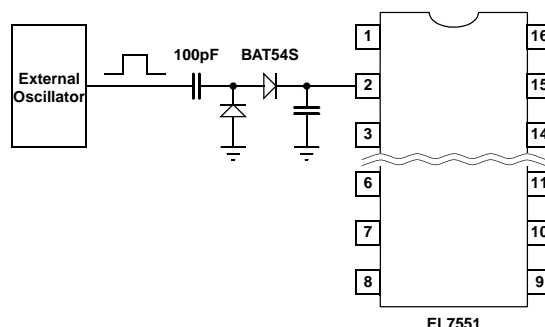
FIGURE 1. OSCILLATOR SYNCHRONIZATION
