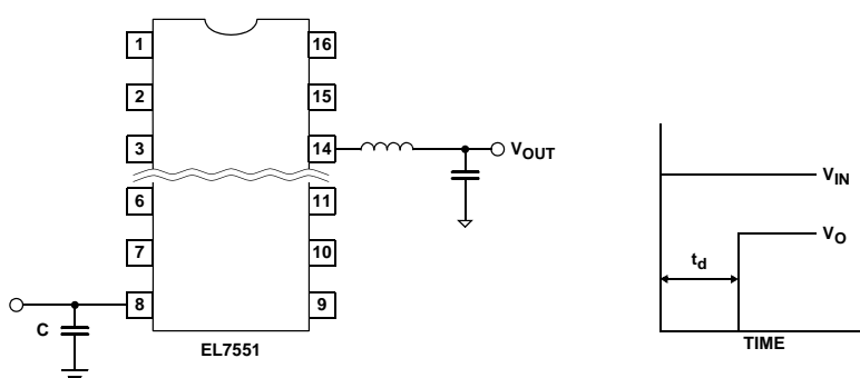
FIGURE 2. START-UP DELAY
