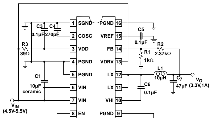
EL7551 (16-PIN QSOP) TOP VIEW
