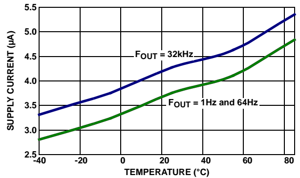
FIGURE 8. I_{DD} vs TEMPERATURE, 3 DIFFERENT F_{OUT}
