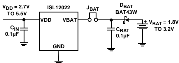
FIGURE 20. SUGGESTED BATTERY-BACKUP CIRCUIT
