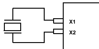
FIGURE 11. RECOMMENDED CRYSTAL CONNECTION
