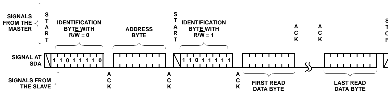
FIGURE 19. READ SEQUENCE (CSR SLAVE ADDRESS SHOWN)
