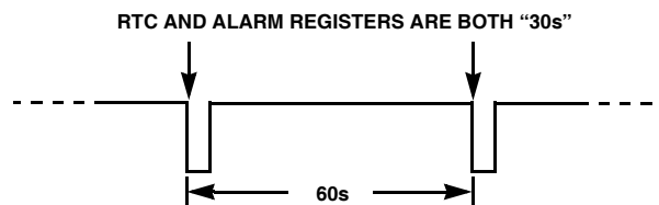
FIGURE 14. \overline{IRQ}/F_{OUT} WAVEFORM
