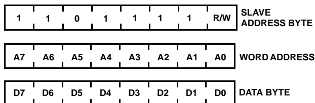
FIGURE 18. SLAVE ADDRESS, WORD ADDRESS, AND DATA BYTES
