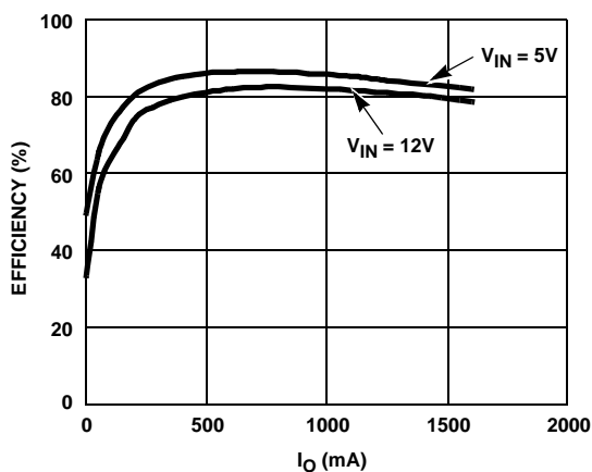
FIGURE 3. BUCK EFFICIENCY
