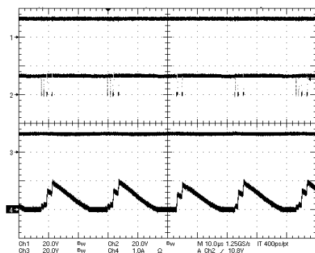
FIGURE 11. BOOST CONVERTER PULSE-SKIPPING MODE WAVEFORM
