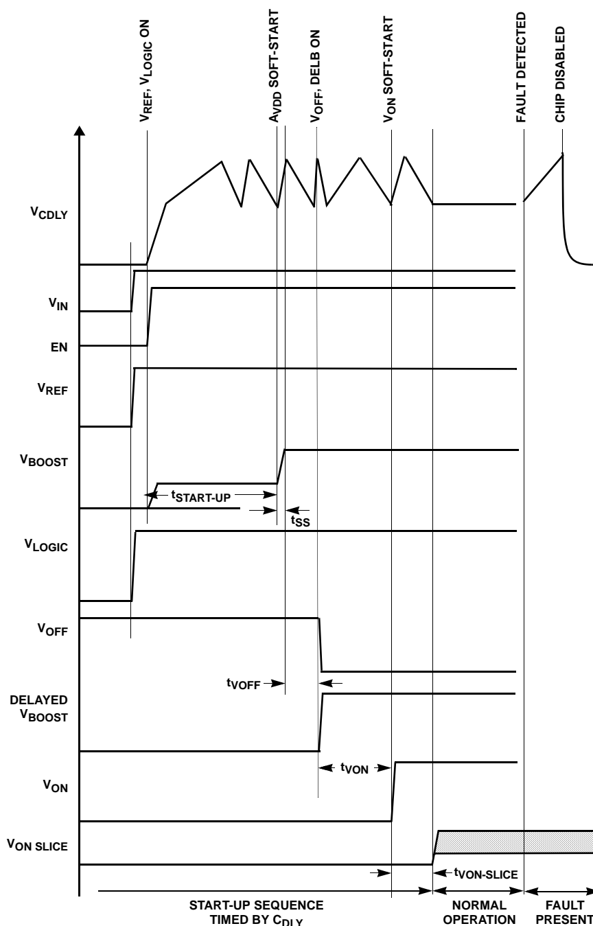
FIGURE 18. START-UP SEQUENCE
