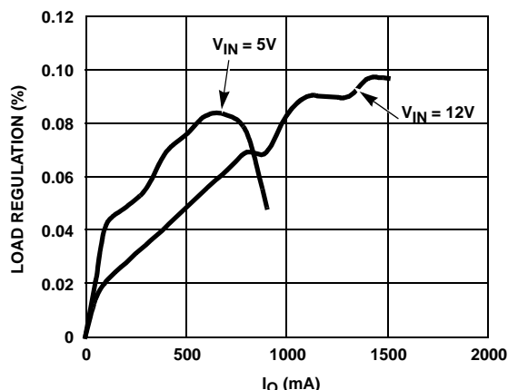
FIGURE 2. BOOST LOAD REGULATION
