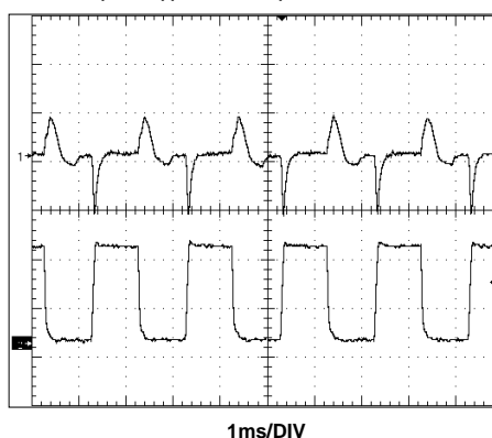
FIGURE 12. TRANSIENT RESPONSE OF BOOST
