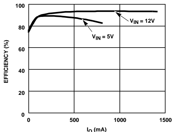
FIGURE 1. BOOST EFFICIENCY
