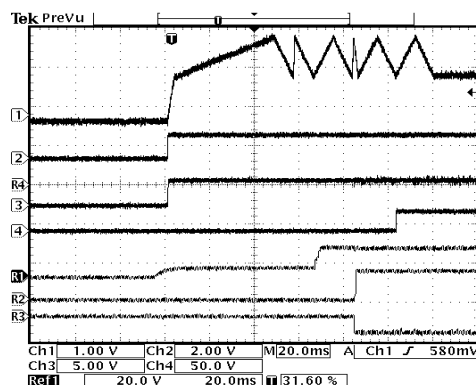
FIGURE 14. START-UP SEQUENCE
