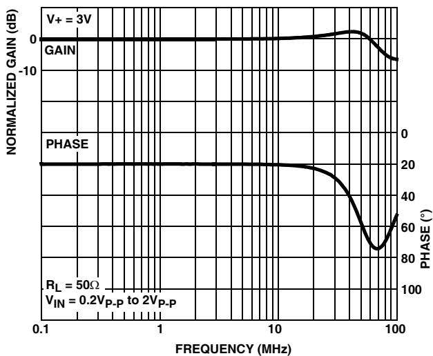
FIGURE 12. FREQUENCY RESPONSE
