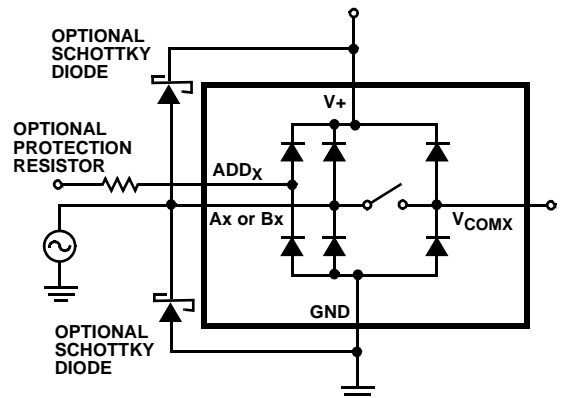
FIGURE 7. OVERVOLTAGE PROTECTION
