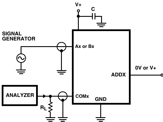
FIGURE 3. OFF ISOLATION TEST CIRCUIT
