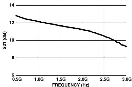
FIGURE 3. |S21| vs FREQUENCY
