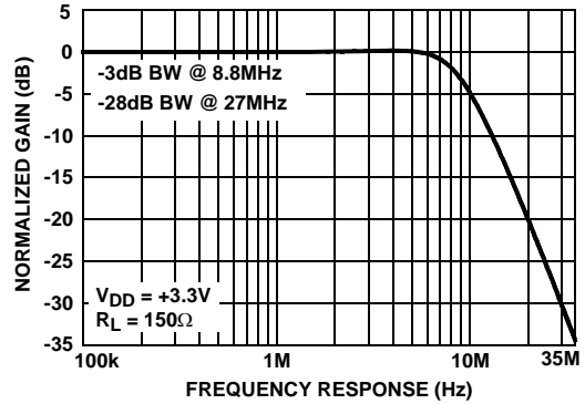
FIGURE 2. GAIN vs FREQUENCY -3dB POINT
