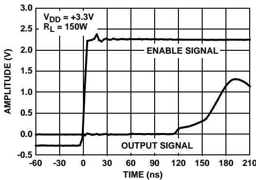
FIGURE 13. ENABLE TIME
