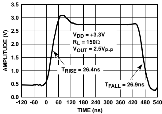
FIGURE 11. LARGE SIGNAL STEP RESPONSE
