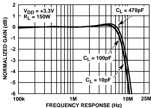
FIGURE 3. GAIN vs FREQUENCY FOR VARIOUS C L LOAD
