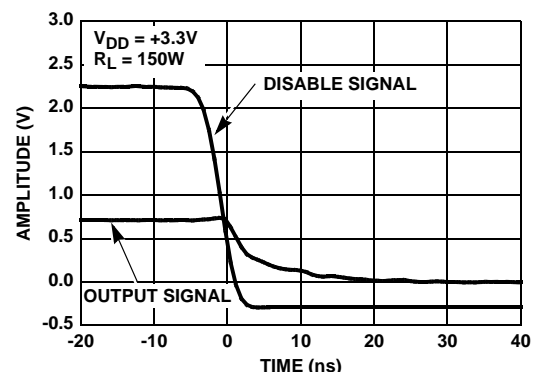
FIGURE 14. DISABLE TIME
