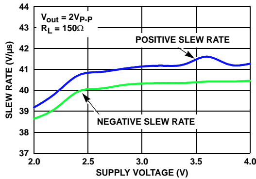
FIGURE 19. SLEW RATE vs SUPPLY VOLTAGE
