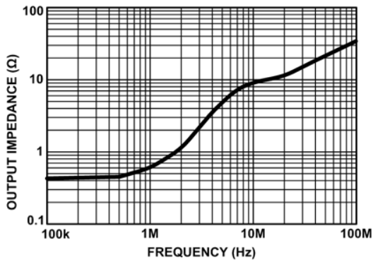
FIGURE 7. OUTPUT IMPEDANCE vs FREQUENCY
