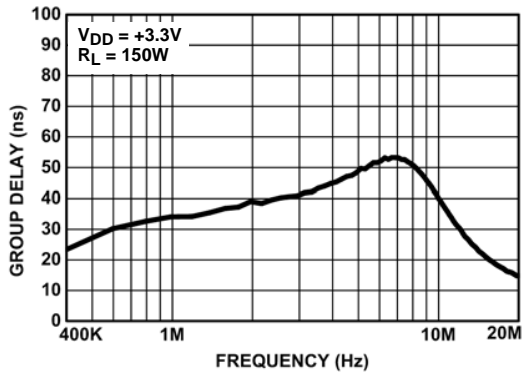
FIGURE 17. GROUP DELAY vs FREQUENCY
