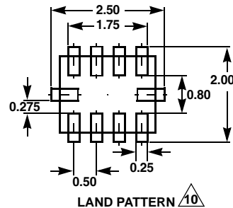
LAND PATTERN
