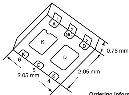
PowerPAK SC-70-6 Dual
