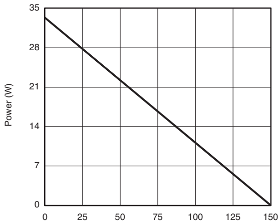
Power, Junction-to-Case
