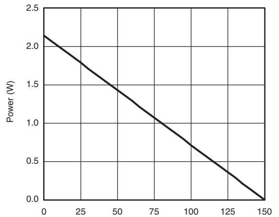
Power, Junction-to-Ambient
