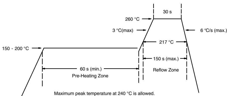
Fig. 4 Solder Reflow Temperatures and Time Durations
