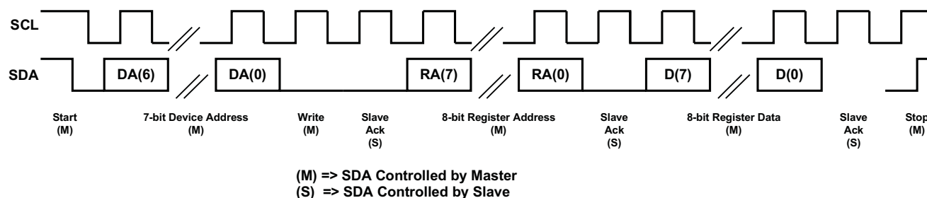
Figure 46. I²C Write
