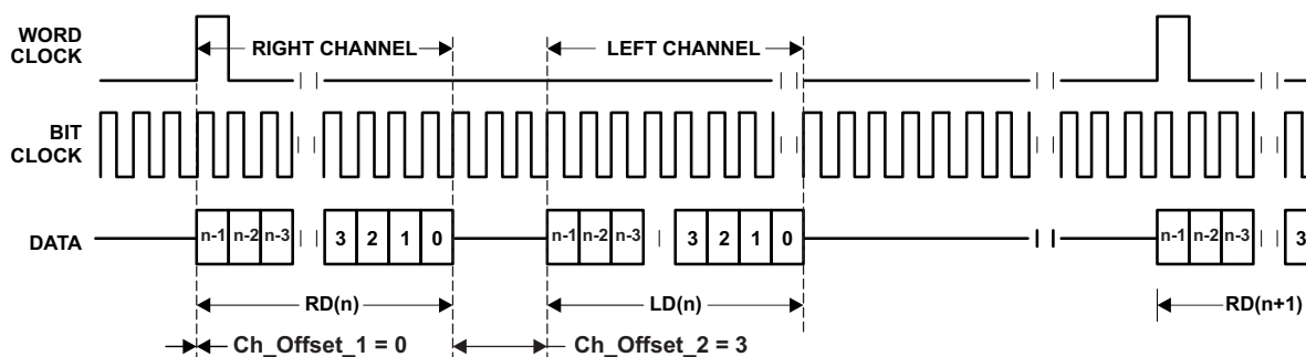
Figure 26. DSP Mode, Time-Slot-Based Mode Enabled, Ch_Offset_1 = 0, Ch_Offset_2 = 3
