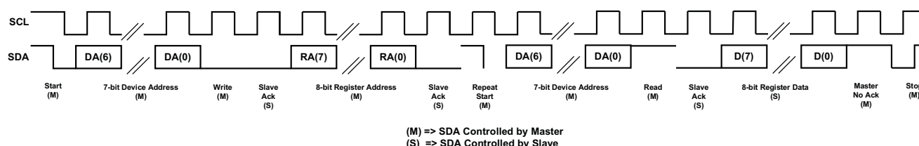
Figure 47. I²C Read
