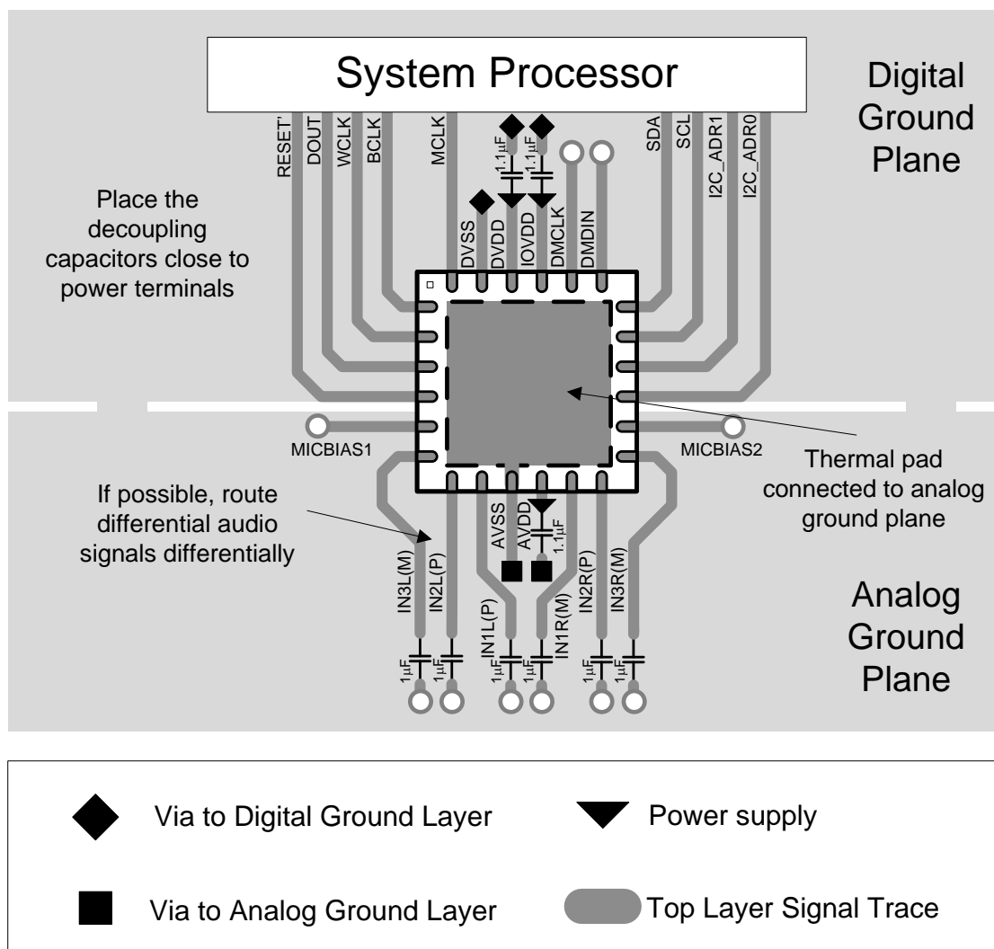
Figure 49. Layout Recommendation
