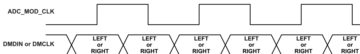
Figure 45. Timing Diagram for Digital Microphone Interface
