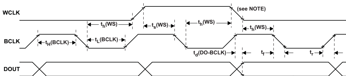
Figure 4. DSP Timing in Slave Mode
