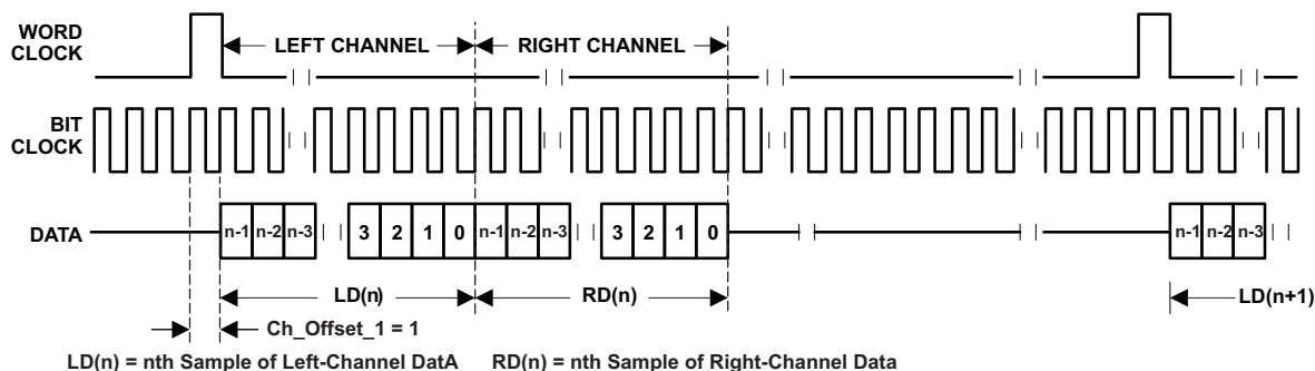
Figure 24. DSP Mode With \text{Ch\_Offset}_1 = 1
