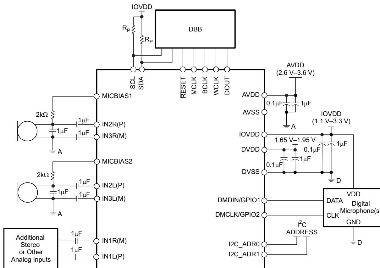
Figure 48. Typical Connections
