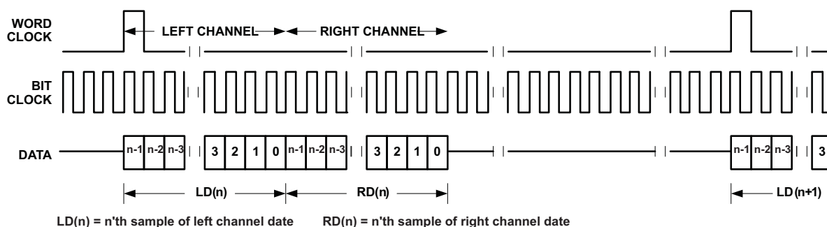
Figure 23. DSP Mode (Standard Timing)
