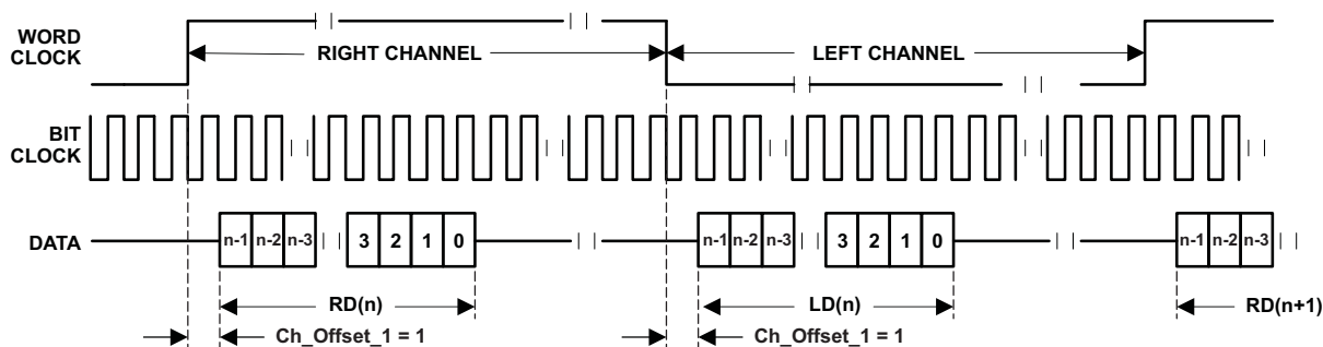
Figure 17. Left-Justified Mode With Ch_Offset_1 = 1, Channel Swapping Enabled
