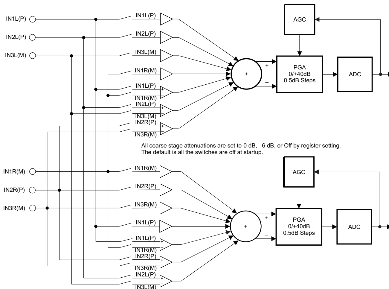
Figure 30. TLV320ADC3101 Available Audio Input Path Configurations
