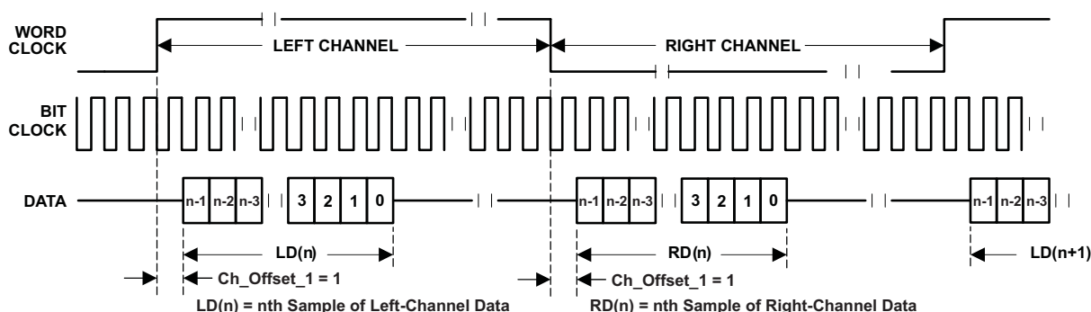
Figure 15. Left-Justified Mode With Ch_Offset_1 = 1
