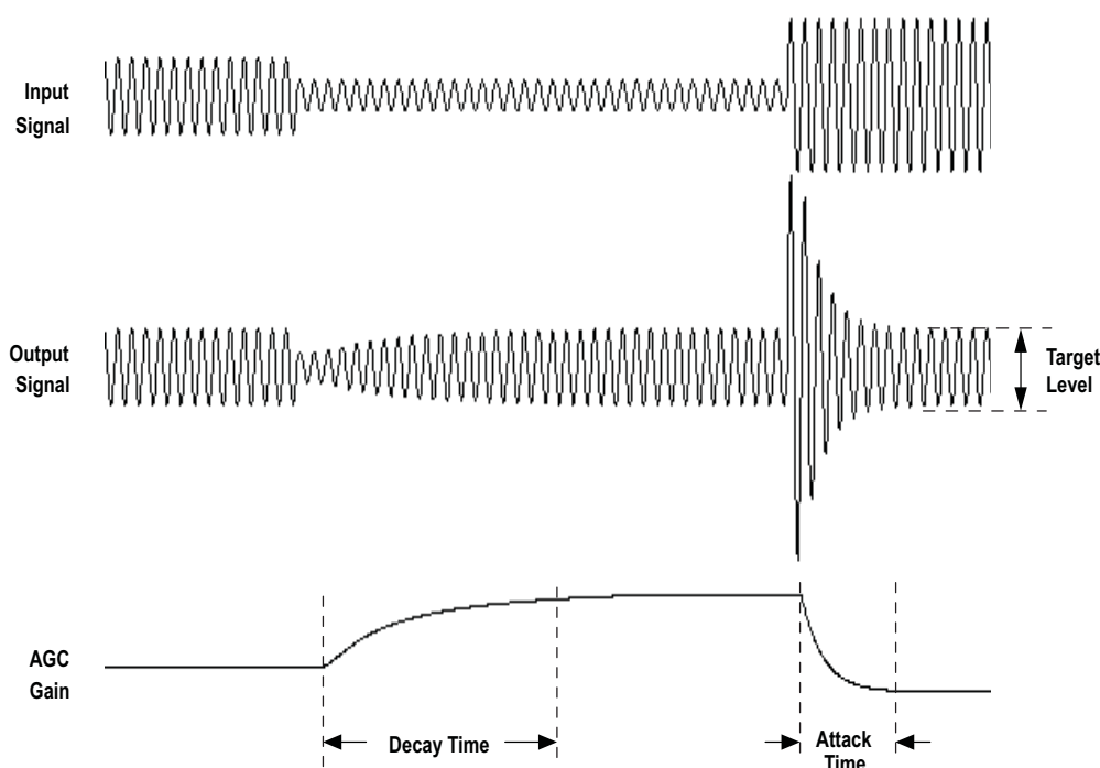
Figure 29. AGC Characteristics
