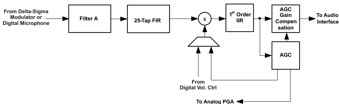
Figure 33. Signal Chain for PRB_R3 and PRB_R6
