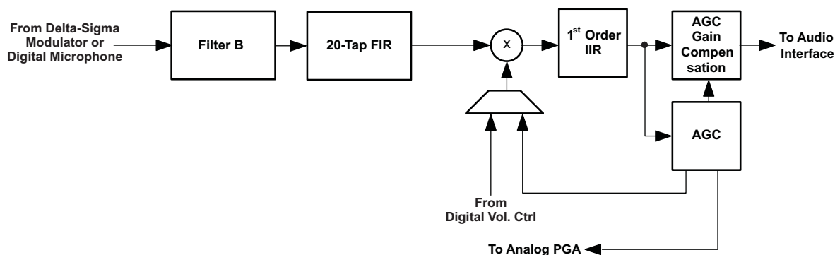
Figure 36. Signal Chain for PRB_R9 and PRB_R12
