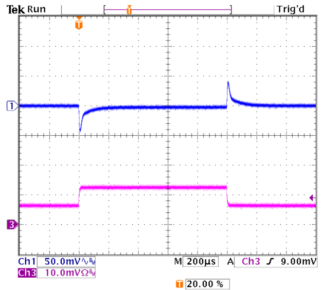
Figure 9. Transient Response to Dynamic Load Change from 40% to 80% of full load (Vin=12V, Vo=1.2Vdc). Ch3 – Iout. Scale=0.2A/mVΩ
