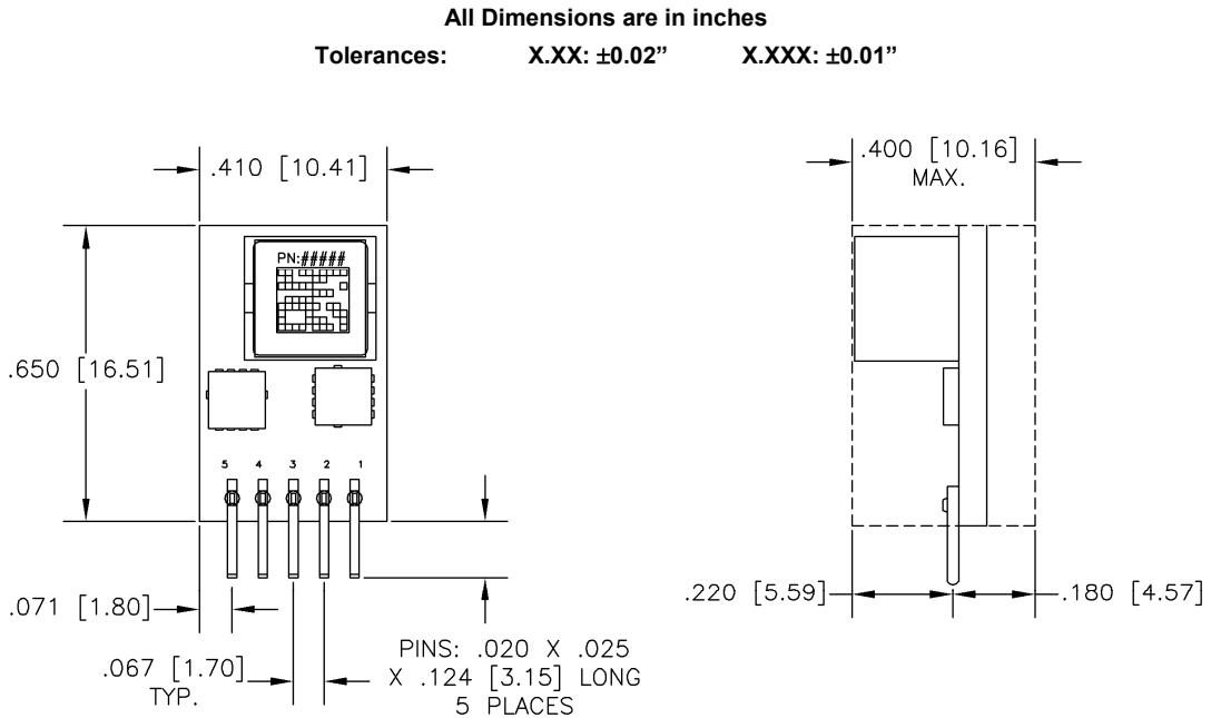
Figure 15. Mechanical Drawing
