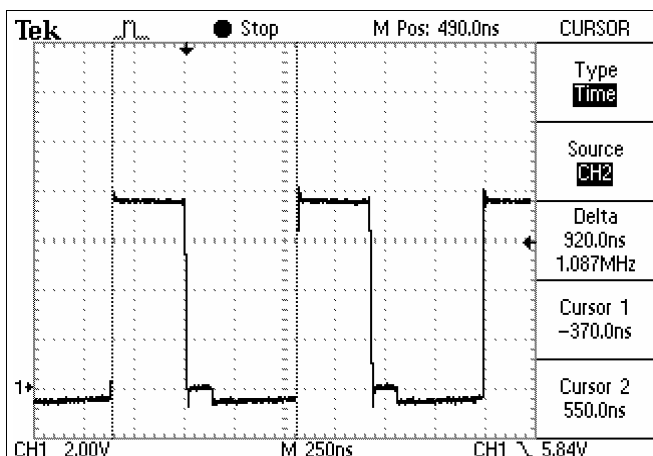
Figure 21. Precharge Waveform
