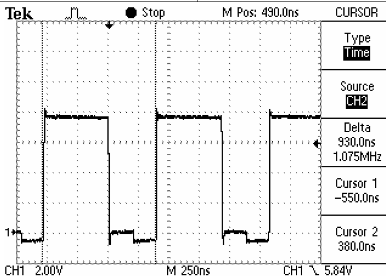
Figure 23. Voltage Regulation and Approaching Termination Waveform
