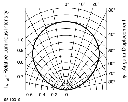
Fig. 3 - Relative Luminous Intensity vs. Angular Displacement
