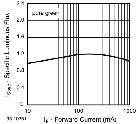
Fig. 26 - Specific Luminous Intensity vs. Forward Current
