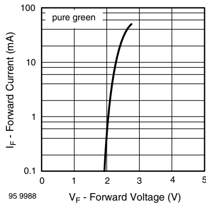
Fig. 24 - Forward Current vs. Forward Voltage
