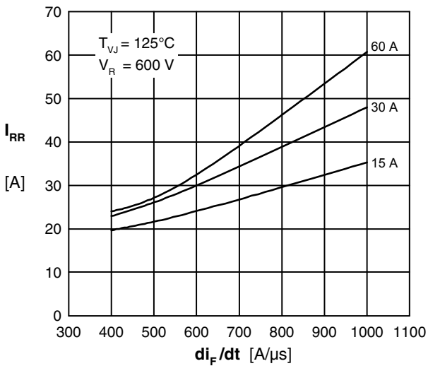
Fig. 3 Typ. peak reverse current I_{RR} vs. di/dt
