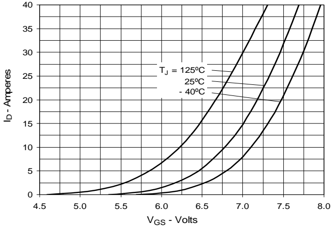
Fig. 7. Input Admittance
