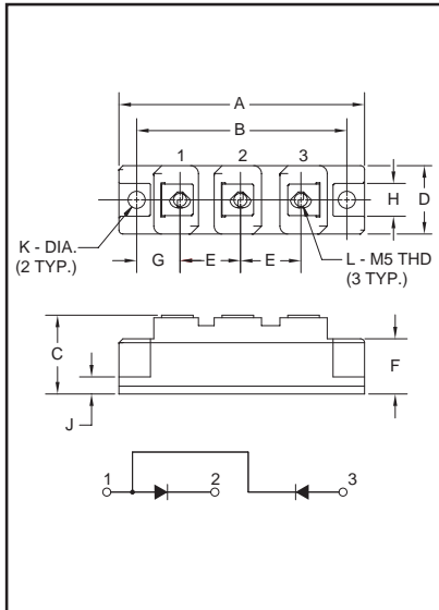
Outline Drawing
