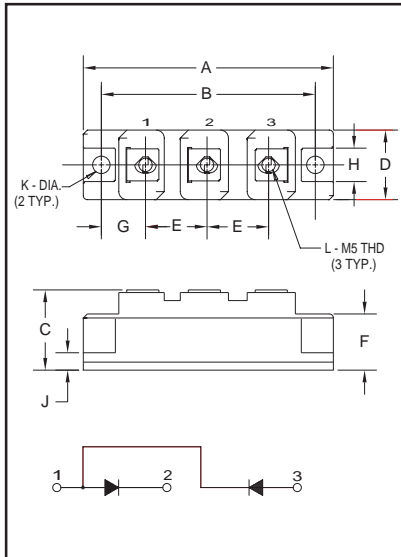
Outline Drawing
