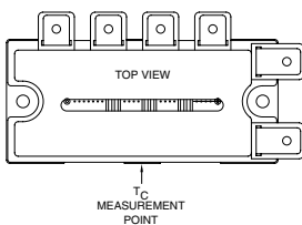
Note 1: T_C (Base Plate) Measurement Point
