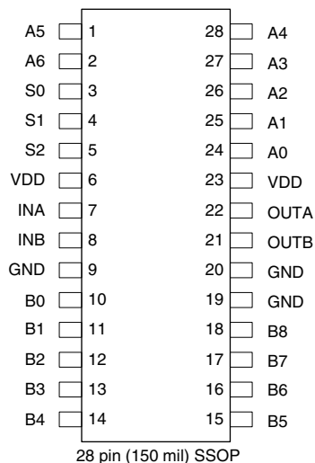
28 pin (150 mil) SSOP
