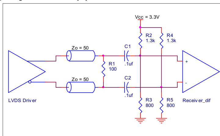
FIGURE 5. DIFFERENTIAL DUTY CYCLE IMPROVEMENT
