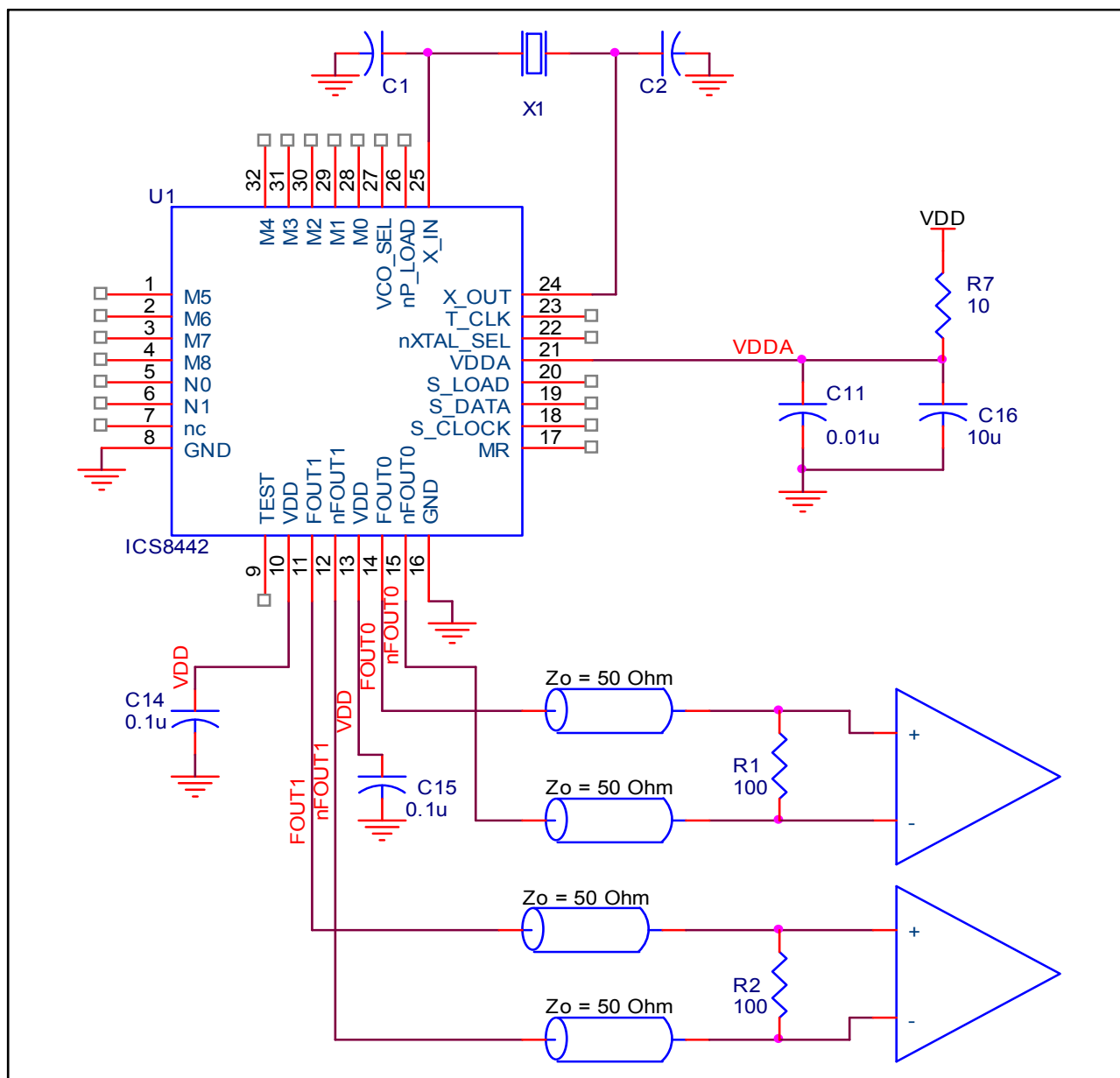
FIGURE 5A. RECOMMENDED SCHEMATIC LAYOUT
