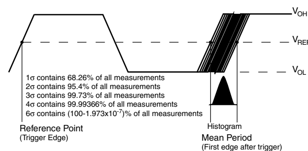
Period Jitter
