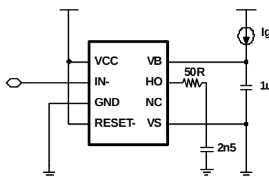
Figure3.b VB Drop Voltage Test Circuit
