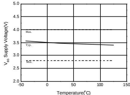
Figure 10b. VBS Under Voltage Threshold(-) vs Temperature
