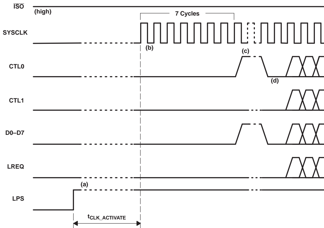
Figure 21. Interface Initialization
