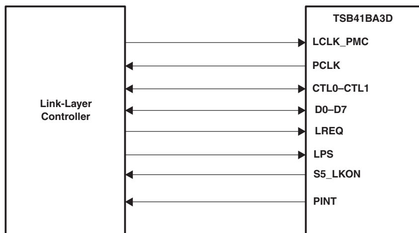
Figure 22. PHY-LLC Interface
