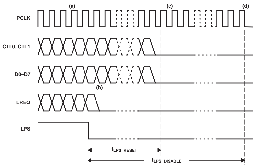
Figure 20. Interface Disable
