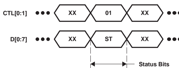
Figure 24. Bus Status Transfer Timing
