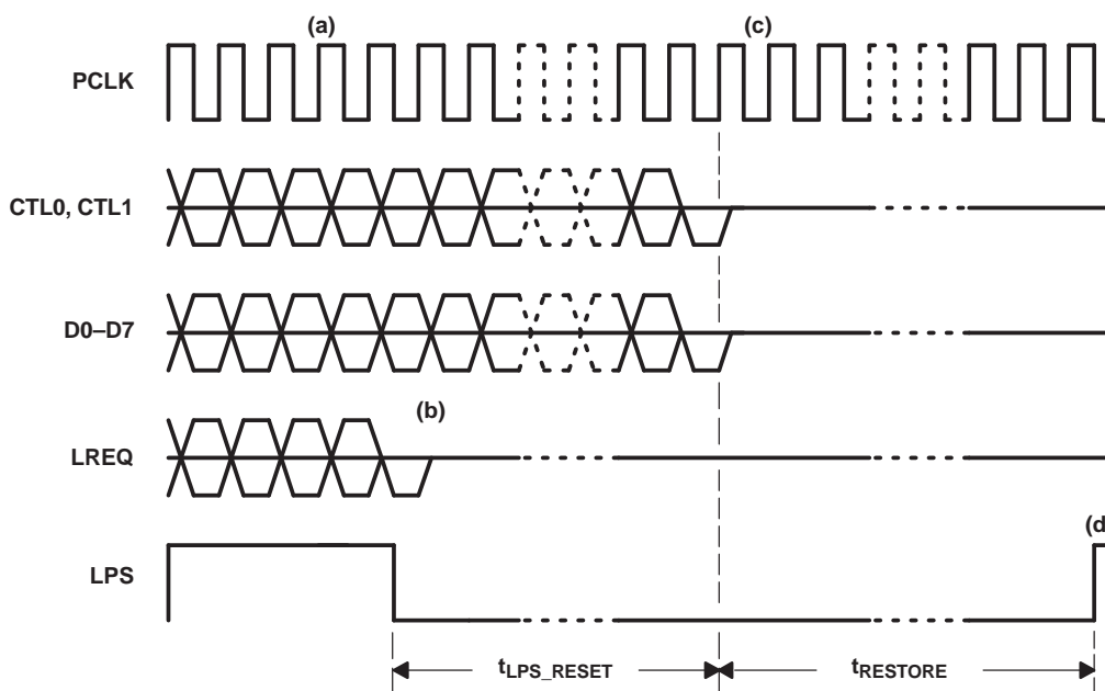
Figure 19. Interface Reset
