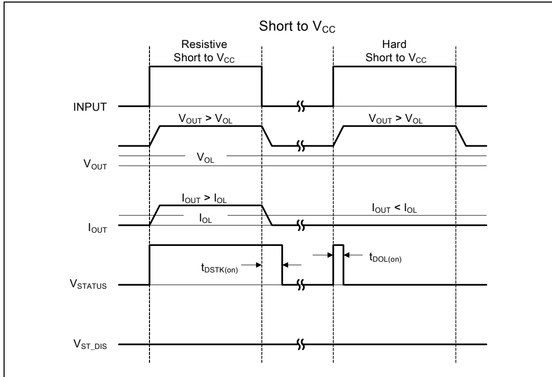
Figure 13. Short to V CC
