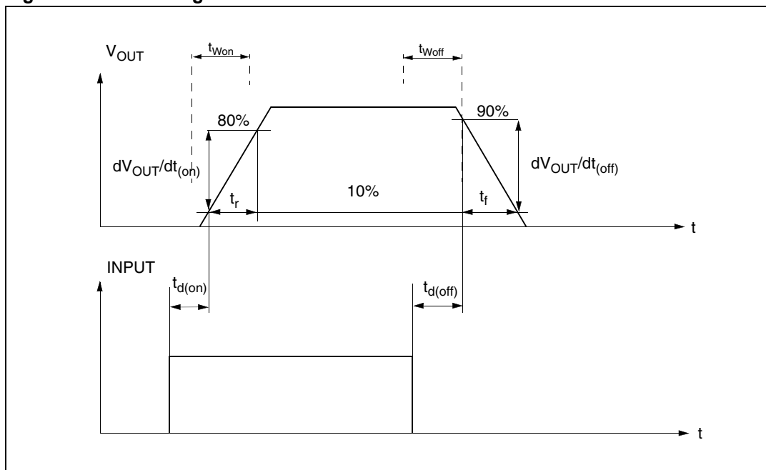
Figure 6. Switching characteristics
