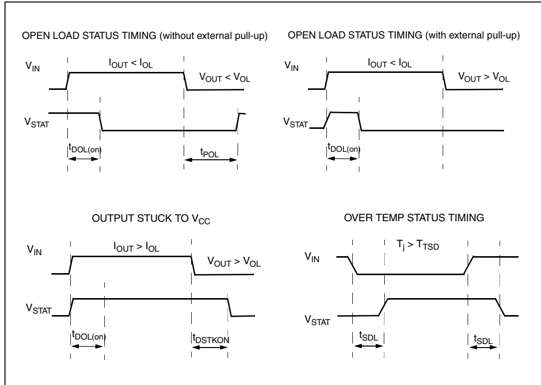
Figure 4. Status timings
